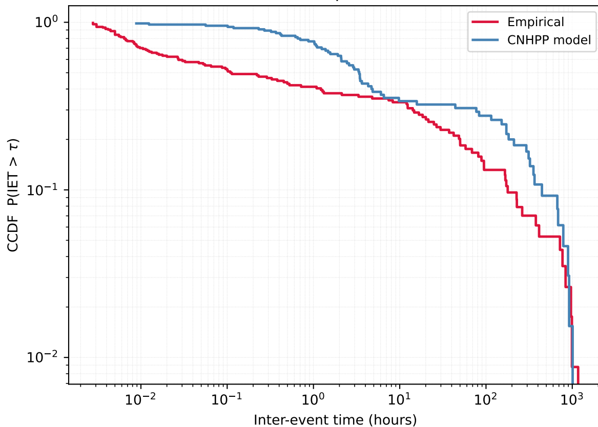
User 5719413972 - Empirical vs CNHPP model
